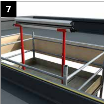
Prop ridge in position using suitable supports, centralising between eaves beam sections. (When the ridge features aluminium painted intenal finish it will need to be protected whilst supporting).
