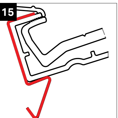
Spring clips in position.
