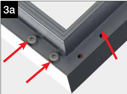
If the pre-drilled holes appear out of alignment as shown above in red simply slacken off the factory fitted screws.
