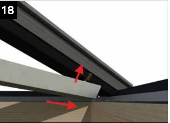
At eaves, slide undercladding down towards eaves as far as you can and push onto clips. Hip claddings are asymmetric. Fit with short cut between hips as shown, claddings have red and blue coloured dots attached to indicate position - always use a red and blue dot at each ridge end.
