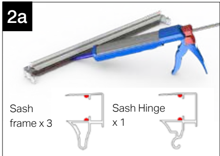
For pitches below 10° it is recommended that the glass is sealed in by running a bead of silicone along the length of each sash section as shown above. For pitches above 10° it is advisable to do the same.
