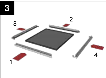
Once tape has been applied, assemble the sash in the sequence shown above and ensure the tape is directed against section 2.
