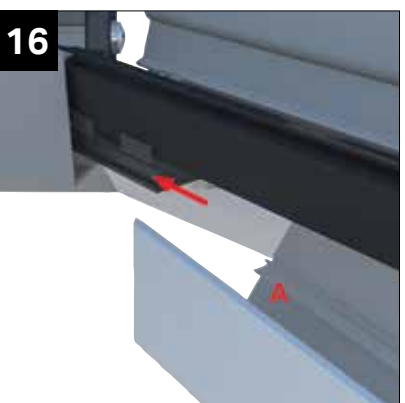
Position top of hips into ridge end ensuring they butt up against it. Locate on the lip as shown above.
