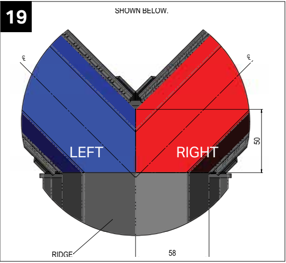
Look up with a 'worms eye view' down the central bar to distinguish left and right.
