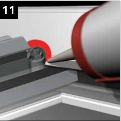
Seal around the notched hip bar top cap ready to receive the jack rafter capping.
