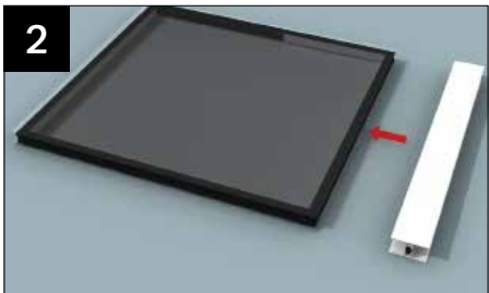
2 IMPORTANT NOTE - APPLIES TO STEPS 7-12. 'H' SECTION GLASS JOINTER TO BE POSITIONED AS INSET ILLUSTRATION ON INSET 1. Slide the glass jointer onto the upper glass unit. Fit assembled unit into the roof.
