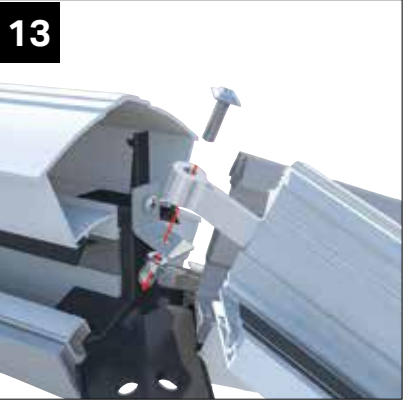
When a transom is fitted between hips, lift transom bar sleeved spigot over bolt, then tighten nut.
