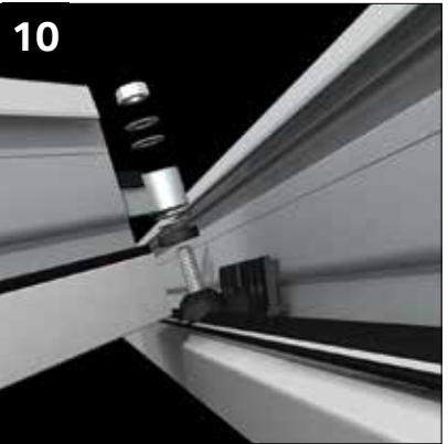
Now fit the jack rafters. The 2 part jack rafter kit is already fitted to the hip and jack rafter. Ease back the jack rafter undercladding. Each jack rafter kit is supplied with a number of washers. Trial fit the jack rafter and check that the glazing platforms are level. Adjust if necessary by adding or removing washers between the two part connecting kit, then tighten the nut. NOTE: If aluminium internal claddings are being used, fit hip internal claddings prior to fitting jack rafters.
