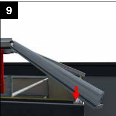
Remove nuts on eaves beam. Fit hip bars onto bolts at eaves end and hand tighten nuts.
