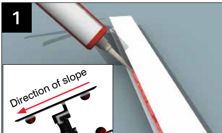
1 Prepare the glass jointer using the appropriate sealant in the four positions shown. This cavity to be upslope.
