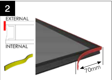
Apply length of foam tape directly to the lower edge of the outer pane of the glass unit as shown. Start by applying the tape 70mm up the side of the glass unit and continuing to wrap around the lower edge of the glass unit, finishing 70mm up the opposite side.
