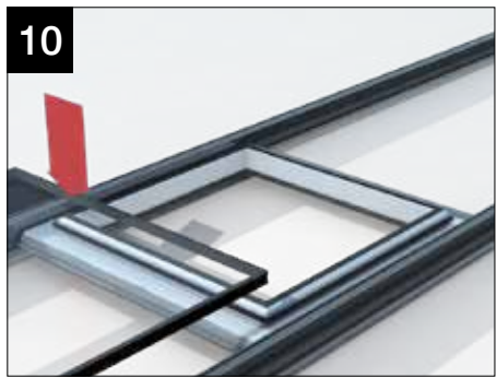
10 Remove any handling tape around the perimeter of the unit. Take care lowering the glazed unit into position on the internal lower muntin bar.
