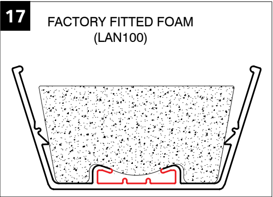
Ensure the foam does not interfere with the clips by pinching it towards the centre of the bar.
