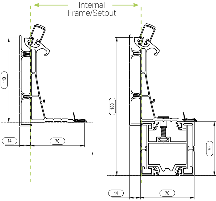
Standard Eaves Beam Bi-fold Support Eaves
