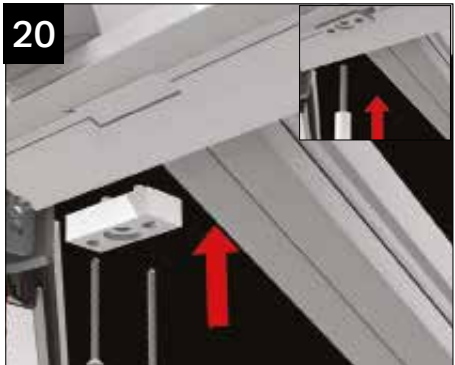
Fix tie bar ridge block to ridge using screws provided. Position by lining up with centre line of bar/brackets. N.B. CLADDING WILL NEED TO BE REMOVED, MARKED AND CUT TO CLEAR BRACKET. Screw tie bar rod into block. Slide tube over rod.
