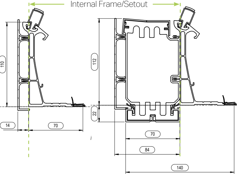
Standard Eaves Beam Super Bolster Eaves
