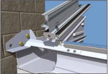
90° EAVES AND RAISED BACK BOX GUTTER ASSEMBLY Place the inline strap (SES005, 165mm / SES006, 265mm) over the single roofing bolt on the sloped gutter. Temporarily fix the bracket to the host wall using three M8 sleeve anchor bolts (SAB001) supplied. Fit the starter bar. Secure the strap to the eaves with the two fixings supplied (UZBGF001-D). Finally, fix anchor bolts.
