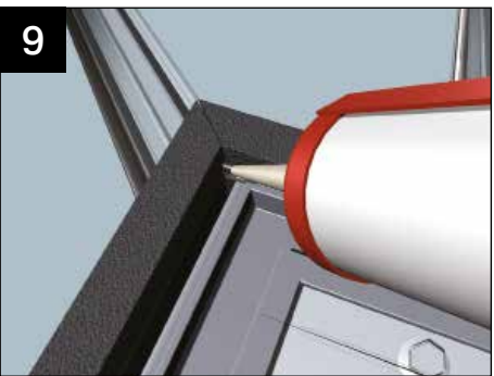
At the corners, seal using a sealant appropriate to the glazing material.
