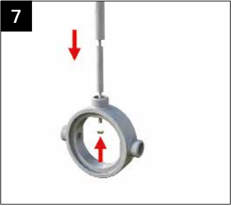
Insert the smaller diameter pieces of pvc conduit inside. Offer into the boss ring and finger tighten the nyloc nut.
