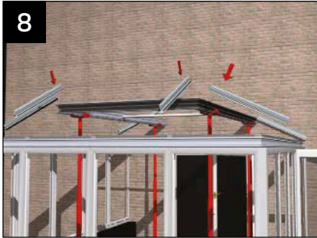
Now the Pagoda eaves beam is assembled into a one piece structure, temporarily support it. Attach the glazing bars according to the component location plan. Tighten the bars, at the pagoda beam end first and then at the main eaves beam second. At the corners, seal using a sealant appropriate to the glazing material (shown above).
