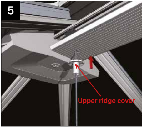
Slide the upper ridge cover over the piece of vertical threaded bar, and insert into the ridge undercladding (the hole may need 'opening' a little – ensure a snug fit).
