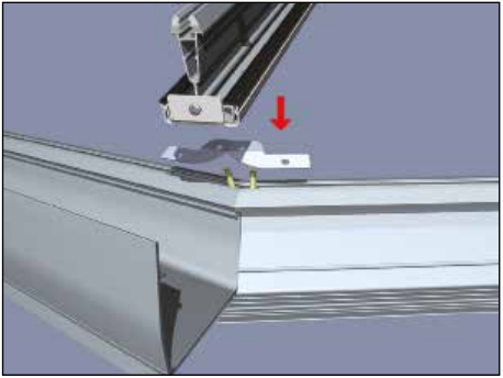
135° EAVES AND BOX GUTTER ASSEMBLY Place the 135° butterfly strap (SES004) over the roofing bolts. Offer the glazing bar on to the bolts, align and secure. Once in position fix the strap down with the two fixings supplied (UZBGF001-D).
