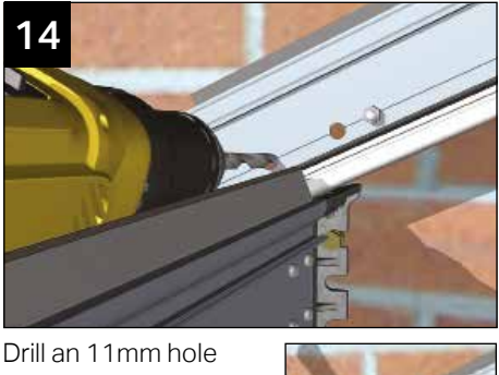
Drill an 11mm hole through the aluminium starter and its factory inserted reinforcement. Then use a 10mm masonry drill bit for the host masonry. IT IS IMPORTANT THAT AN ANCHOR BOLT GOES INBOARD AND OUTBOARD OF THE EAVES BEAM.
