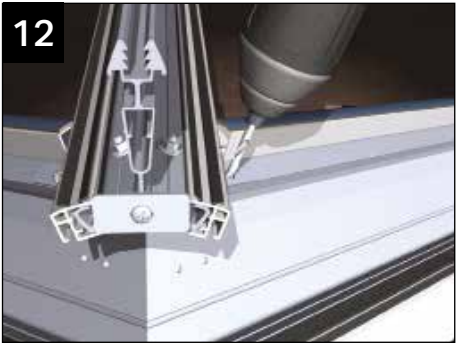
Drill a 5.5mm hole either side and then fix the 'butterfly' cleat into the head of the eaves beam at the 90 degree corners using the fixing provided.
