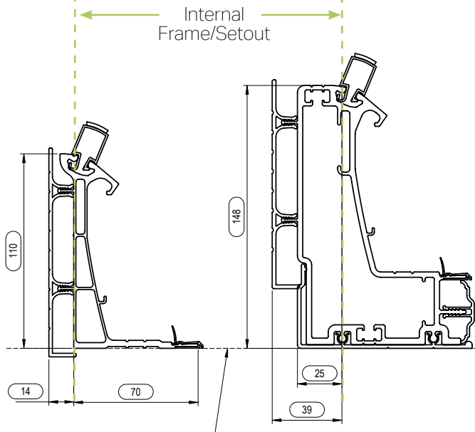
Standard Eaves Beam Super Duty Eaves Beam
