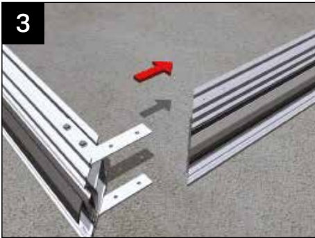
Slide the cleated corners into the adjacent piece of lantern beam
