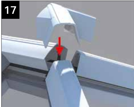
Press firmly down on the ridge end top cap until it clicks into position on the ridge end.
