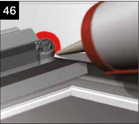
Seal around the notched Georgian top cap ready to receive the jack rafter capping.
