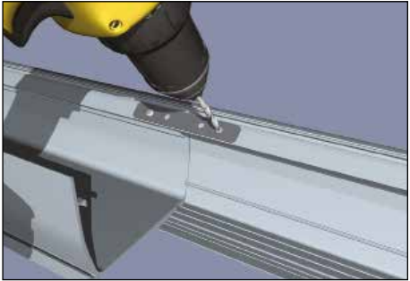
180° INLINE EAVES AND BOX GUTTER ASSEMBLY Place the inline cleat (SES002) over the butt joint. Fix down either side of the joint with the two fixings supplied (UZBGF001-D).
