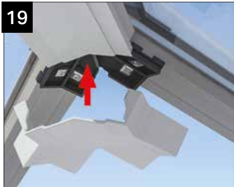
Fit the internal plastic cover if supplied by pushing up into position over the ridge and ridge end.
