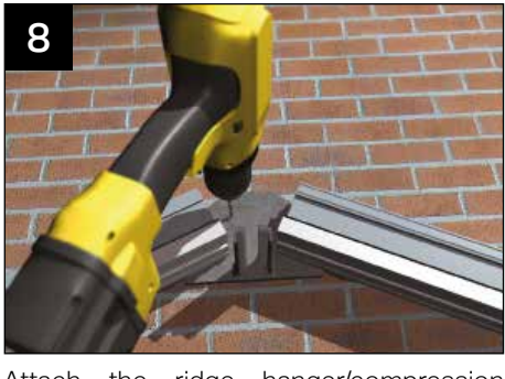
Attach the ridge hanger/compression plate to the host wall. Drill the plate with 2 x 9mm holes, then the wall with an 8mm masonry bit and fasten into the masonry using the two M6 x 65mm sleeve anchors (or resin anchors) provided. If necessary, use aluminium shims to pack out behind the plate. Check the plate is vertical and securely fastened. AT THIS STAGE IT IS ADVISABLE TO CHASE OUT FOR CONSERVAFLASH /LEAD FLASHING.
