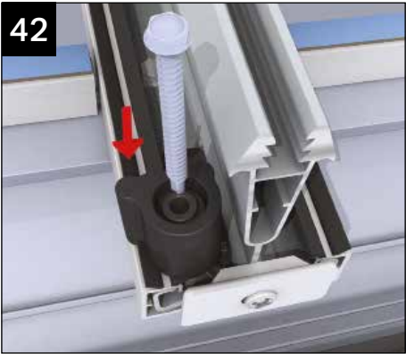
Ensure the glazing end profile sits snugly behind the grommet. Now, using the fixing provided screw down into the bar as shown. Ensure clip offers maximum support to glazing at all times.
