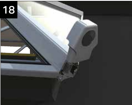
Fit end caps to bars and push in circular cover disk to finish.
