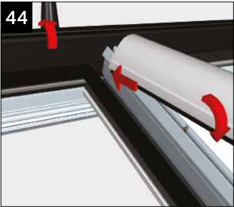
Work your way around the roof. The top cap must be lifted into its final resting place (at the ridge) prior to being knocked down over the Anchor clip.
