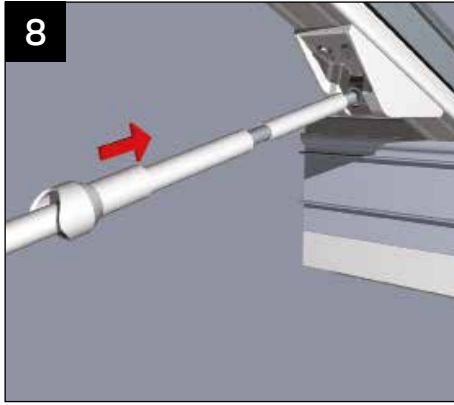
Offer up the horizontal pieces of pvc conduit (large and small diameter).
