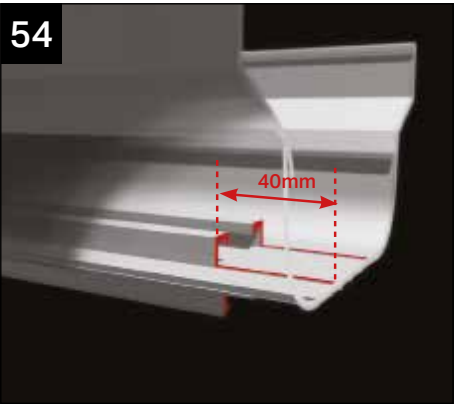
Now for the ridge top cap - Cut back the cresting channel on the top and the T bolt slot on the underside of the ridge top capping by 40mm.
