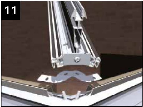
Lay the butterfly cleat over the two captivated roofing bolts. Fit the Georgian hip bar at the eaves and ridge end. Note: A butterfly cleat is not required on 3 or 5 facet fronts unless the eaves beam joins a box gutter at the facet joint. (See image below)
