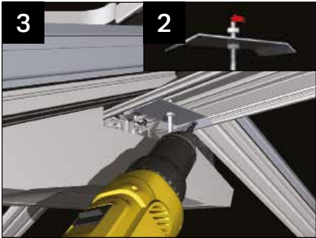
Measure the drop for the vertical threaded bar and cut to length. Attach the gusset plate to the threaded bar with the nyloc nuts provided. Ensure spanner tight. Now fit the gusset plate to the aluminium ridge body using the four screws provided. Make sure it lines up with the centre line of the pre-attached tie bar brackets. At this stage the pvc ridge undercladding needs fitting. Drill an 11mm hole in it and clip the pvc ridge undercladding into place.
