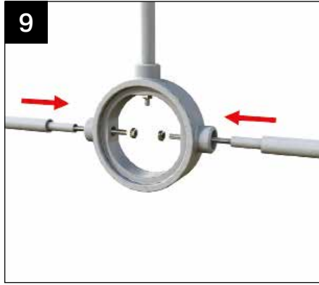
Insert threaded bar into the ring, and again finger tighten the nyloc nuts.
