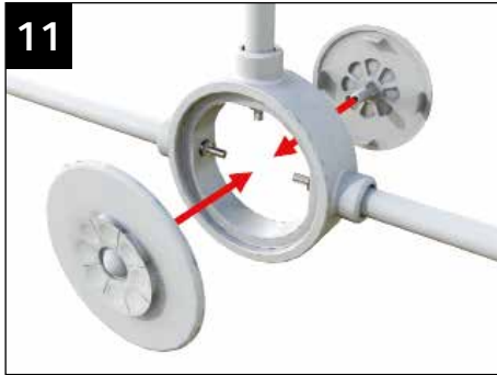
Offer up the two part rose cover, spin one half onto the threaded end of the other half.
