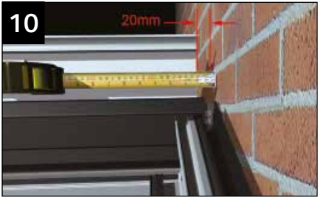
The ridge body should ideally sit 20mm away from the house wall (or 12mm from the front plate), this allows the compression plate to evenly distribute ridge loads into the host wall (max tolerance 50mm). If the host wall is out of plumb, pack out behind the starter bars and use the longer bolts provided. This ensures the starter bars are at 90° to ridge body (and not tapering).
