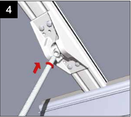
Measure, cut and attach the horizontal threaded bars (ensure sufficient engagement of the bar into the brackets) – it is essential that the tie bar boss is central. Take the boss ring, and loosely assemble the threaded bars to check they terminate inside the ring. Dis-assemble.
