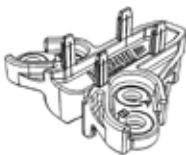
IRK001 INTER RAFTER TENNON IRK002 STRUCTURAL JACK RAFTER BASE KIT IRK003 INTER RAFTER WEATHERING SHIELD IRK005 FLASHING TRIM- RUNNER
